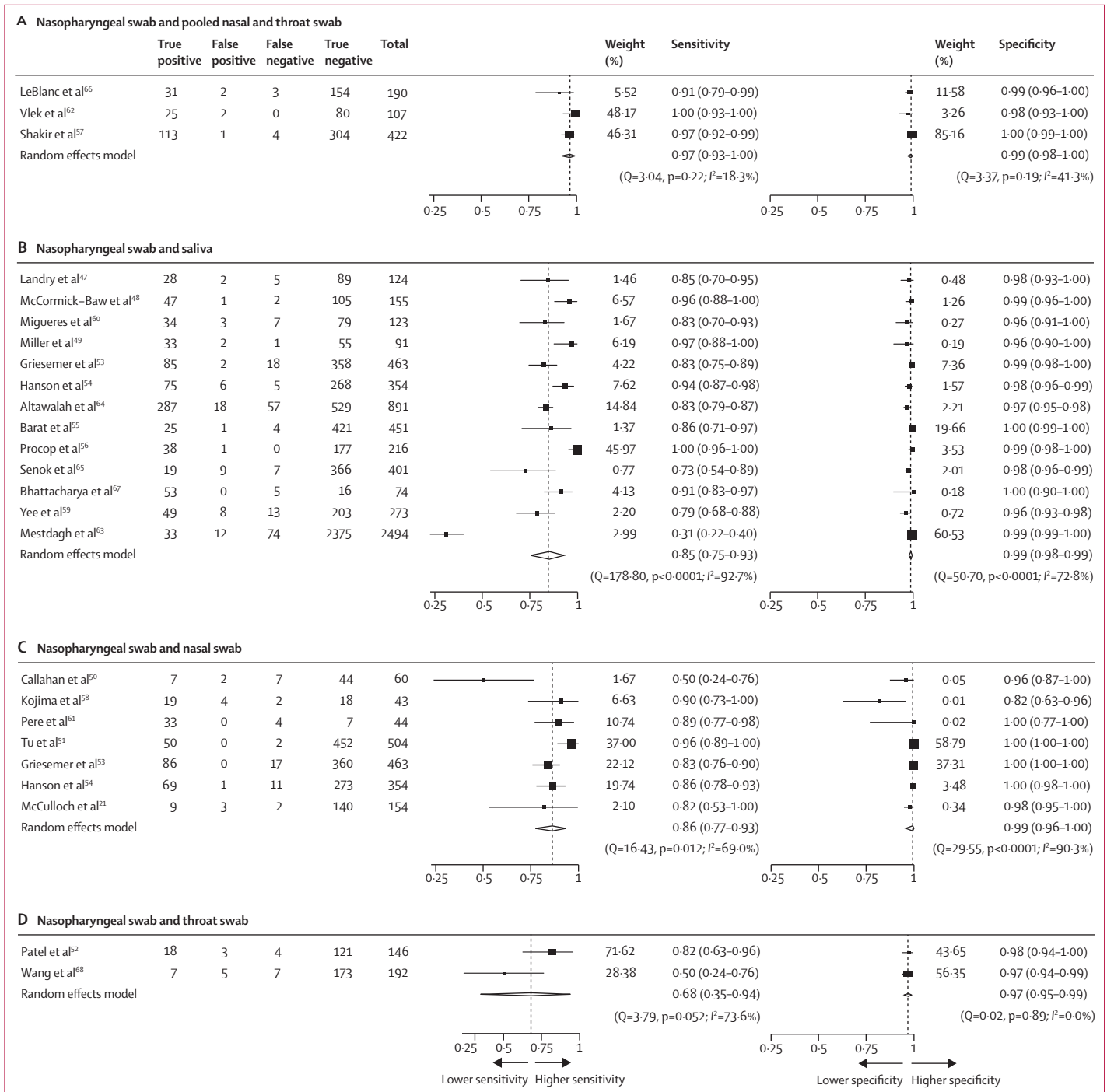
Figure 2: Meta-analysis of the sensitivity and specificity, using nasopharyngeal swab as a reference standard Forest plots of sensitivity and specificity. Squares (proportional to the sample size, disease prevalence, and heterogeneity) represent point estimates.
